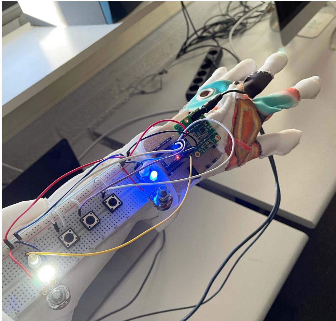
Synthesizer Glove Teensy soundwave library synthesizer Chords (Stretch) Year2023
