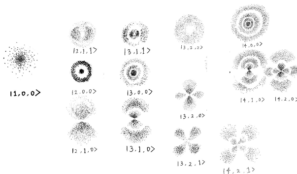
[fig. 1 Hydrogen wave function |(n), (l), (m)\rangle ]
